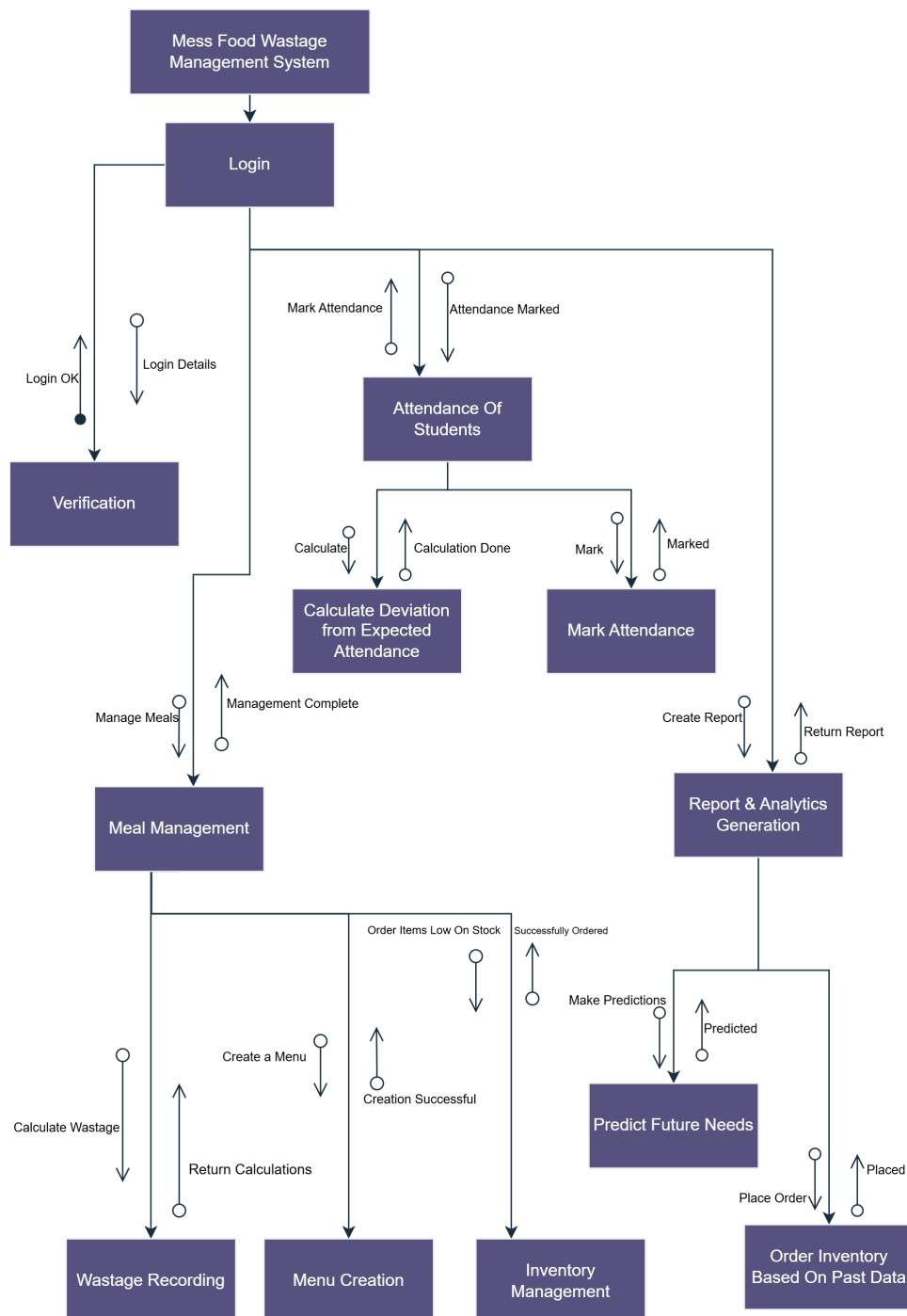
Figure 8.2: Structure Chart
